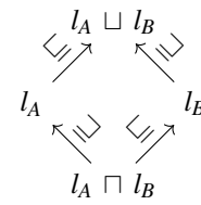
Fig. 3. Simple lattice.
