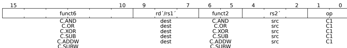
Figure 79: Integer Register-Register Operations (cont.)
