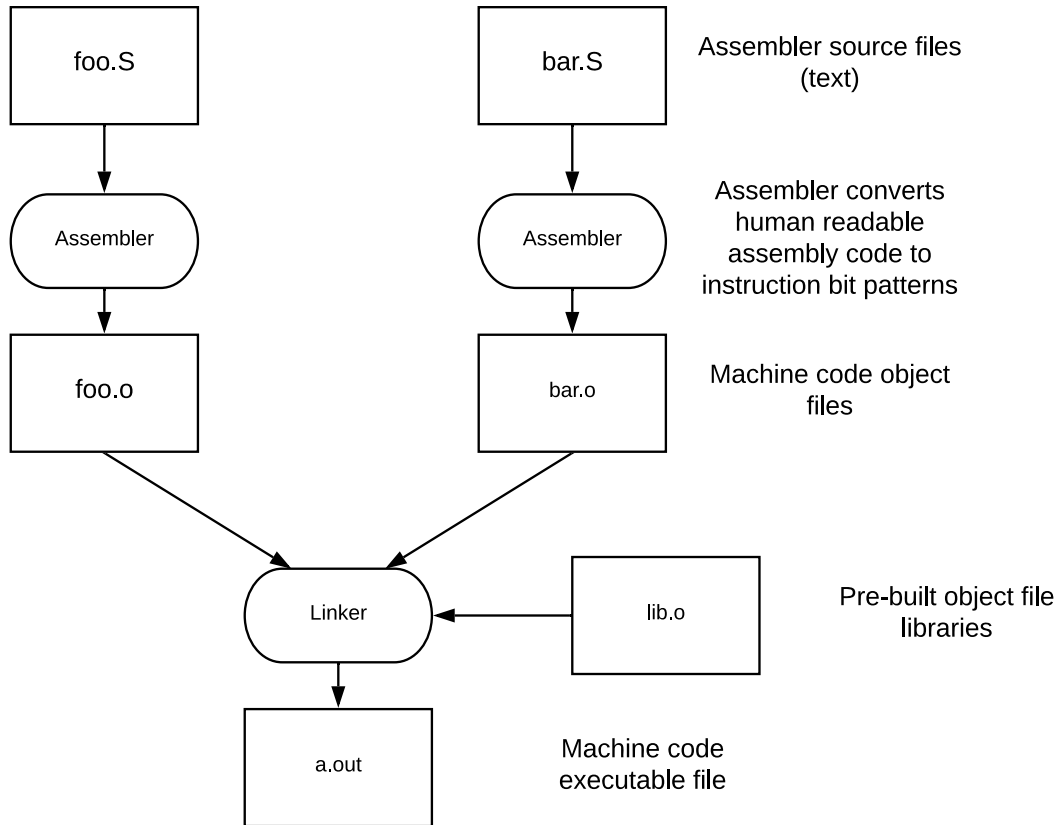
Figure 103: RISC-V Assembly to Machine Code
