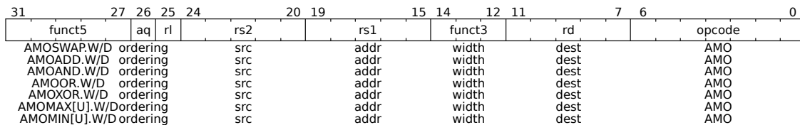
Figure 36: Atomic Memory Operations
