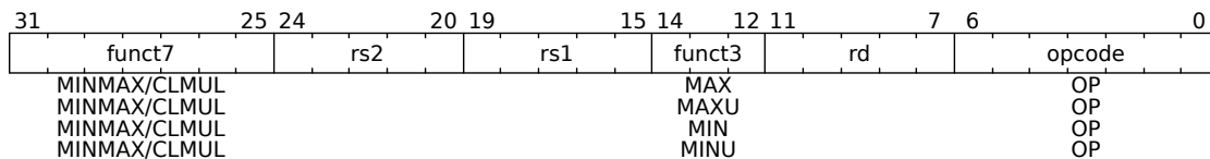
Figure 90: Comparison Instructions
