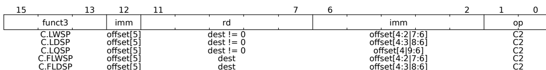
Figure 65: Stack-Pointed-Based Loads
