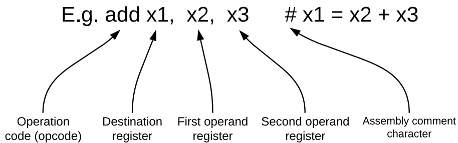
Figure 102: RISC-V Assembly Example
