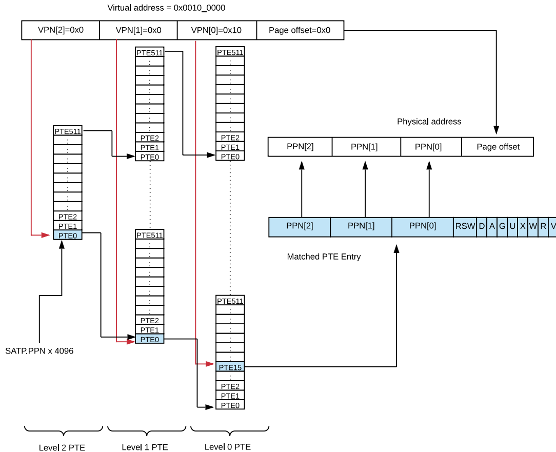
Figure 9: Hardware Table Walk Example
