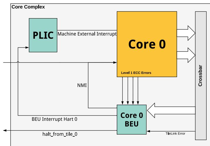
Figure 111: Bus-Error Unit Block Diagram
