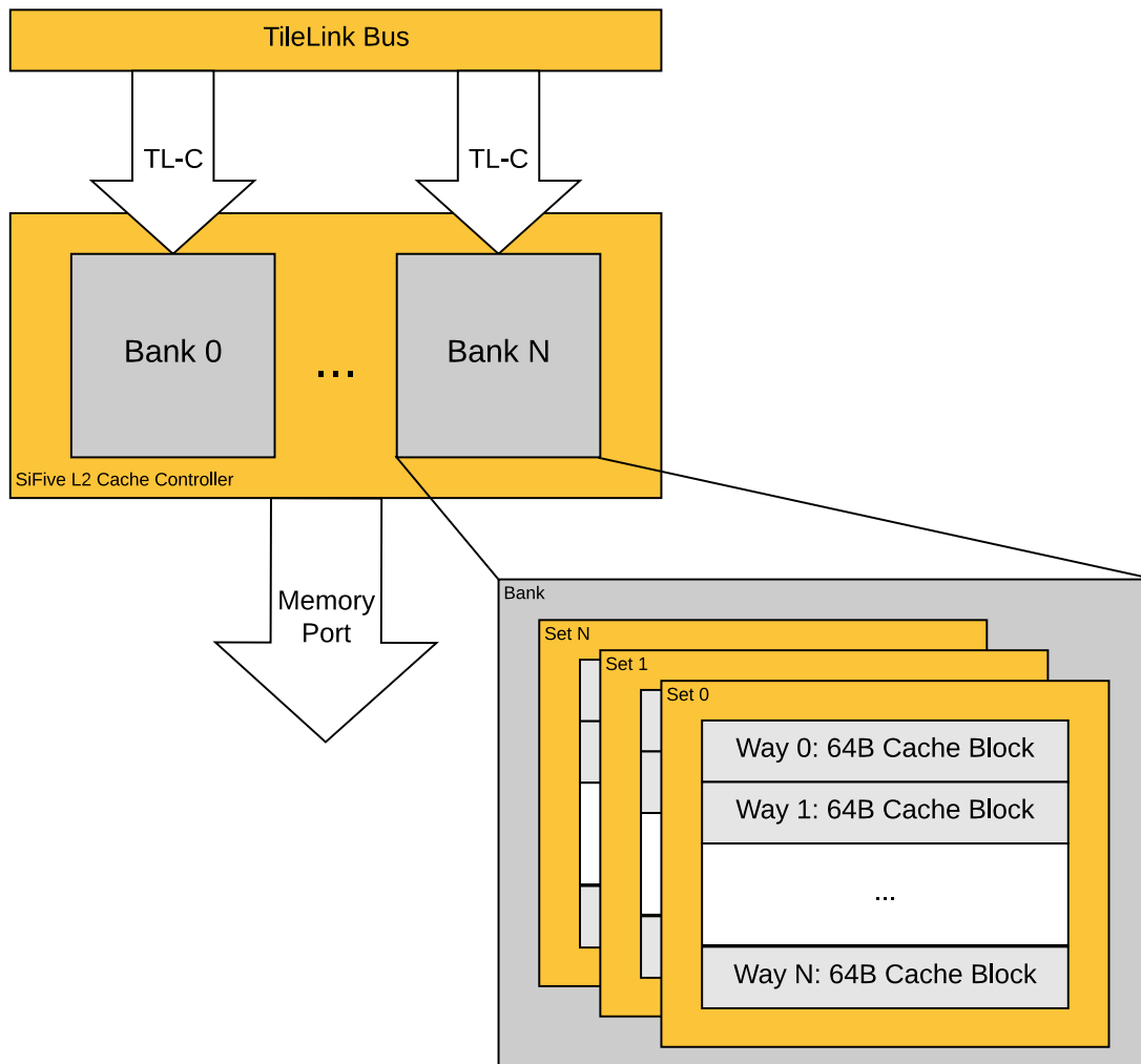
Figure 112: Organization of the SiFive L2 Cache Controller
