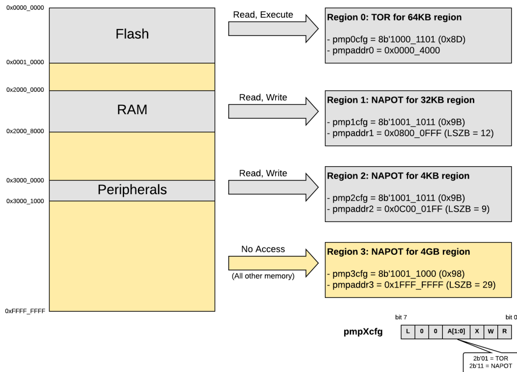
Figure 14: PMP Example Block Diagram
