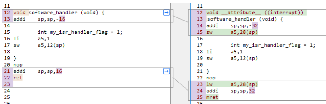
Figure 110: CLINT Interrupt Attribute Example
