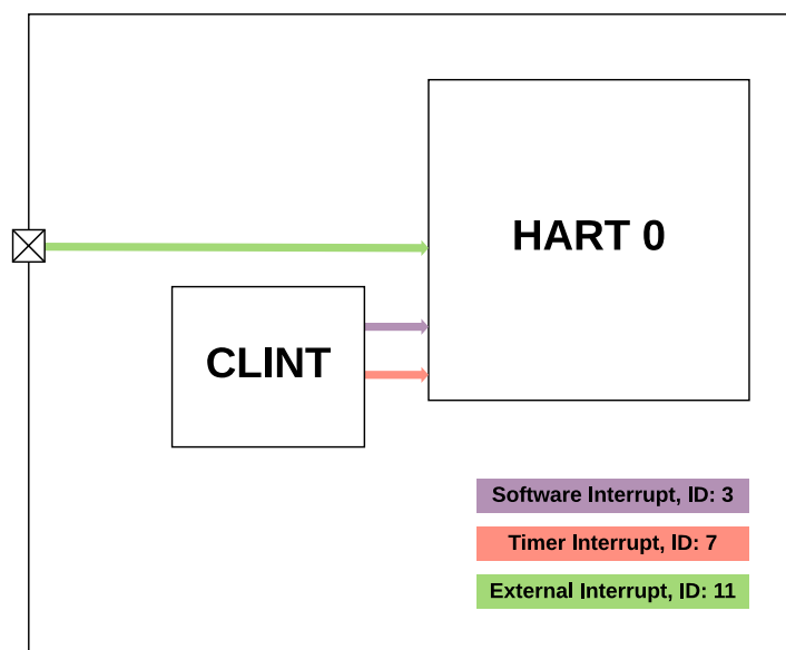
Figure 107: CLINT Block Diagram
