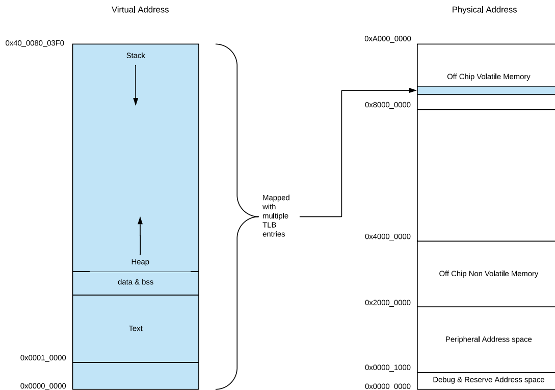
Figure 8: Linux User Application Memory Map Example
