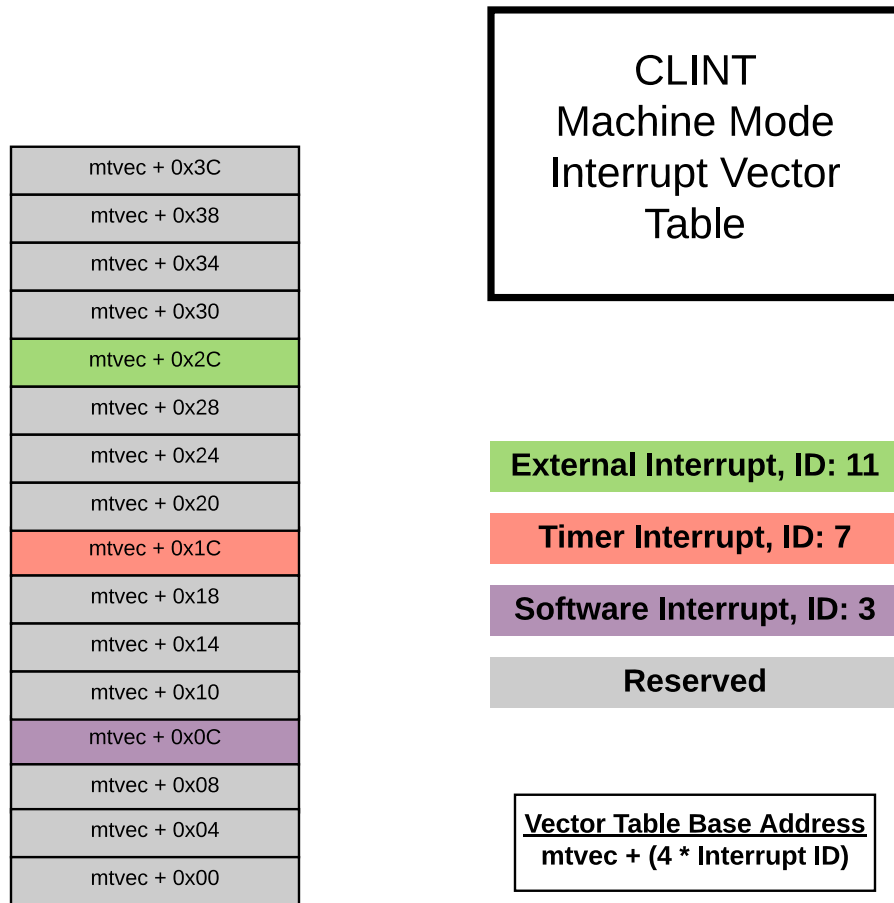
Figure 108: CLINT Interrupts and Vector Table
