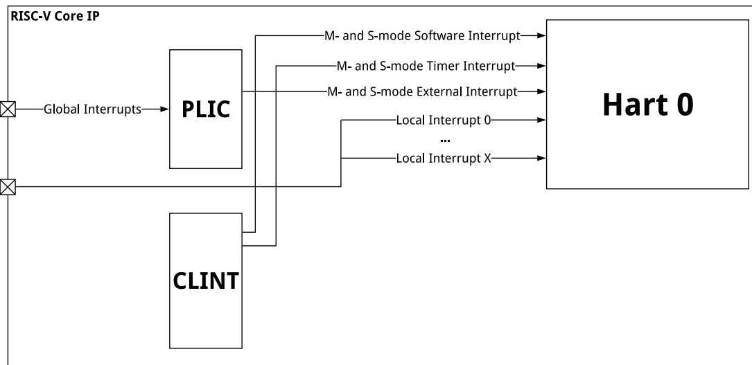
Figure 106: U74 Core Complex Interrupt Architecture Block Diagram
