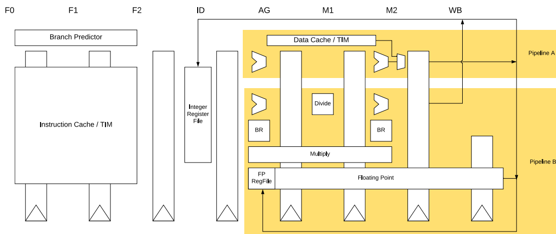
Figure 2: U7 Execution Pipeline
