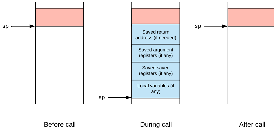
Figure 105: Stack Memory during Function Calls
