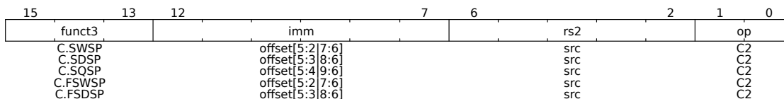
Figure 66: Stack-Pointed-Based Stores
