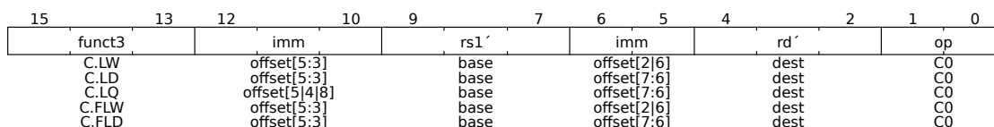
Figure 67: Register-Based Loads
