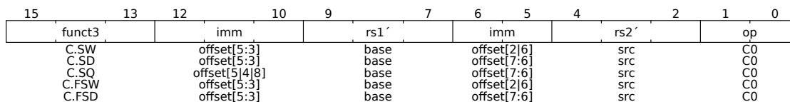
Figure 68: Register-Based Stores
