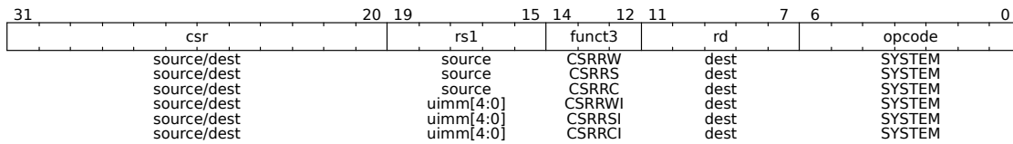
Figure 97: Zicsr Instructions
