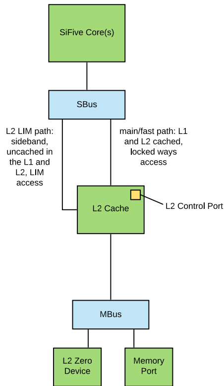
Figure 114: Difference between L2 LIM and L2 Zero Device
