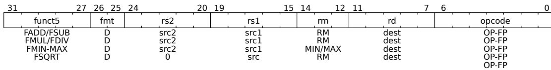
Figure 49: Double-Precision FP Computational Instructions
